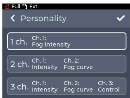
Fig. 26: Setting Personality
